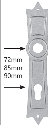
3426601 52x260mm 3mm
