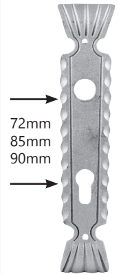
3426801 56x260mm 3mm
