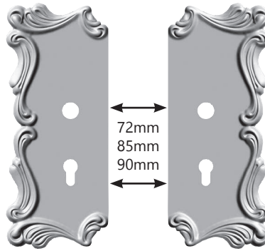
3523401 3523301 133x318mm 133x318mm 2mm
