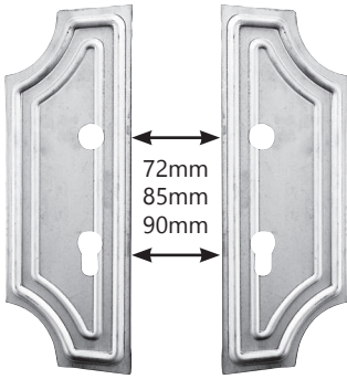
3440101 3440201 104x277mm 104x277mm 2mm
